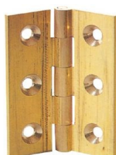
H.202 Brass Butt 1.1/2" x 7/8" (38mm x 22mm) 2" x 1.1/8" (51mm x 28mm) 2.1/2" x 1.3/8" (64mm x 35mm) 3" x 1.5/8" (76mm x 41mm)
