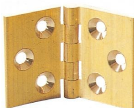
H.1030 Back Flap 1.1/4" x 1.7/8" (32mm x 48mm) 1.1/2" x 2.3/8" (38mm x 60mm) 2" x 3" (51mm x 76mm)
